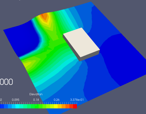
OpenFOAM-4.x, interFoam
