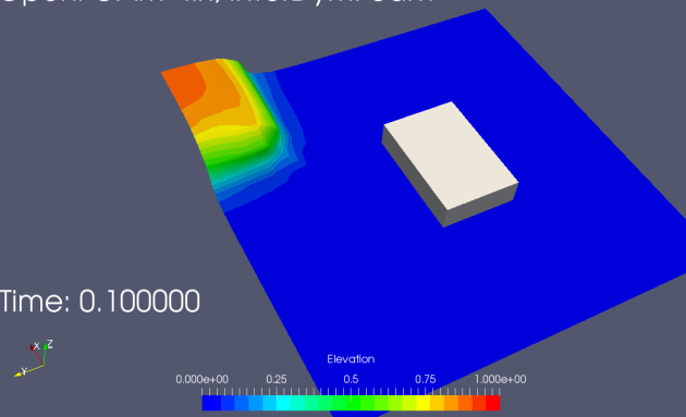
OpenFOAM-4.x, interFoam
